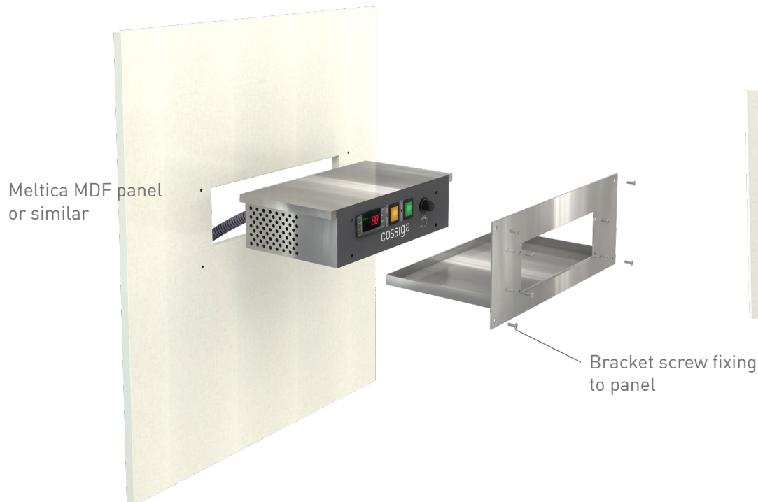
LSCM 4 BRACKET
